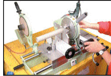
Positioning fitting in clamp
